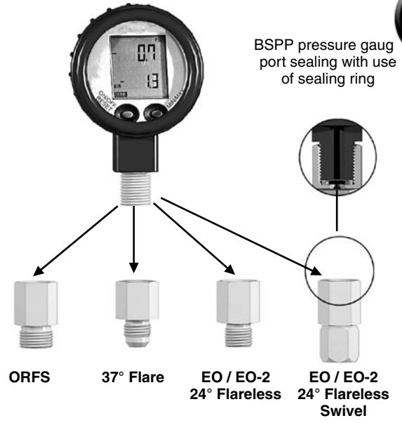
Fig. N4 — BSPP pressure gauge connections
